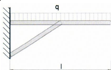
Load diagram
